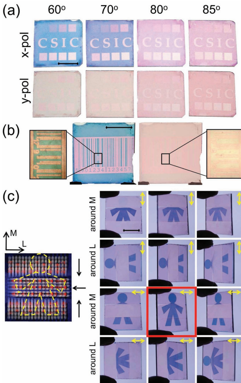
Figure 5. a) Pictures of a series of Au/SiO 2 samples deposited at \alpha = 60, 70, 80 , and 85^\circ illuminated with x- and y-polarized light. Selected zones of these samples were treated with laser at powers ranging from 25 to 95% of the total output power ( 240 \text{ kW/cm}^2 ) at 10% intervals (eight squares in the outer zone of each sample). The central "C S I C" characters have been written by using a laser power of 60%. b) Standard bar code written with the laser onto a Au/SiO 2 -60° sample and monitored with x- and y-polarized lights. The zoom images show the presence of a secondary micrometric bar code engraved in one of the bars. c) Optical effects in an irradiated Au/SiO 2 -60° sample with three different orientations of the nanocolumns. The scheme illustrates the different orientations of the gold nanoparticles in the original sample and the contour of a figure written by laser irradiation. The photographs on the right correspond to the irradiated sample illuminated with x- (top figures) and y- (bottom images) polarized lights and turned by 90° around the axis perpendicular to the film and by approximately \pm 45^\circ around the axis in the film plane as defined in the scheme at the left side of the figure (L and M axis). The arrows at the right of this scheme indicate the incoming direction of the material flux during the preparation of each part of the sample. The scale bar included in the upper left picture corresponds to 1 cm.
